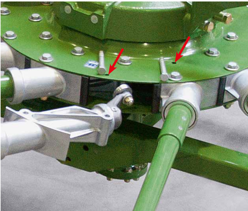
Each tine arm is easily removed Simply undo two bolts to remove the entire arm complete with bearing and roller.
